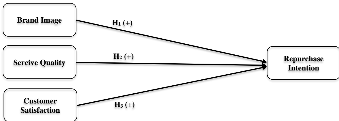
Figure 1. Research Framework
