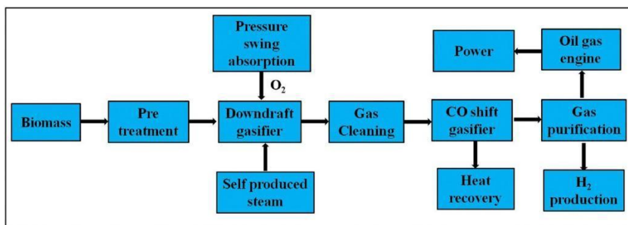
Fig.6. Flow diagram of the biomass hydrogen production process.
